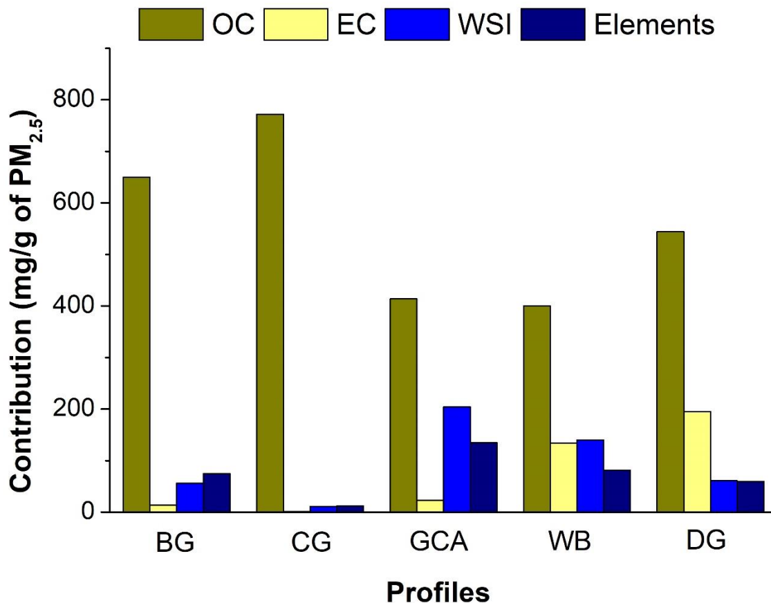
323 Fig. 1: Contribution of OC, EC, water-soluble ions (WSI), and elements to reconstructed PM_{2.5} 324 emitted from the different sources (BG: beef grilling, CG: chicken grilling, GCA: general 325 cooking activities, WB: wood burning, DG: diesel generator).
