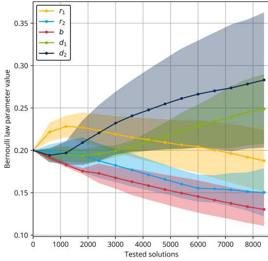
Figure 4: Evolution of mutation rate vector's coordinates during the run, using method AMOW.
