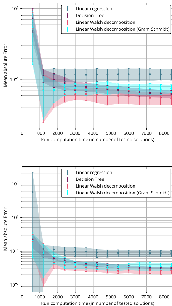
Figure 3: Mean absolute error on f_1 (top) and f_2 (bottom) obtained from different surrogate methods during a run. The training dataset is updated each 600 tested solutions.
