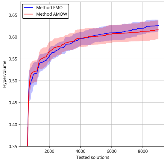
Figure 5: Evolution of hypervolume referenced to the origin of the objective space for method FMO (fixed mutation operator) and AMOW (adaptive mutation operator based on Walsh decomposition). Hypervolume was computed thanks to the library (López-Ibáñez et al., 2010).
