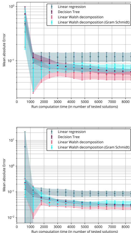
Figure 3: Mean absolute error on f_1 (top) and f_2 (bottom) obtained from different surrogate methods during a run. The training dataset is updated each 600 tested solutions.
