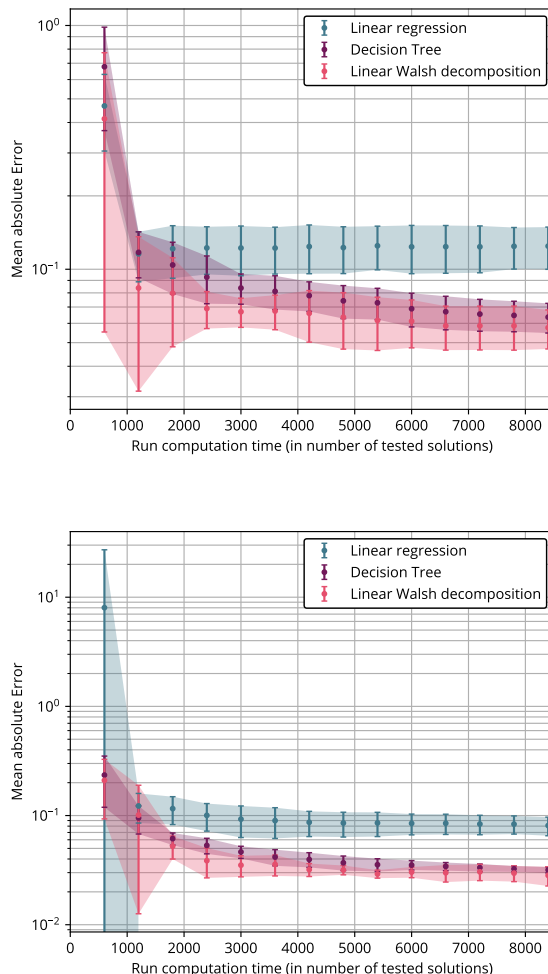
Figure 3: Mean absolute error on f_1 (top) and f_2 (bottom) obtained from different surrogate methods during a run. The training dataset is updated each 600 tested solutions. Points stand for mean values over all runs whereas shaded areas stand for the 1\sigma confidence interval (note that y-axis scale is logarithmic so mean values are not centered in error bars).
