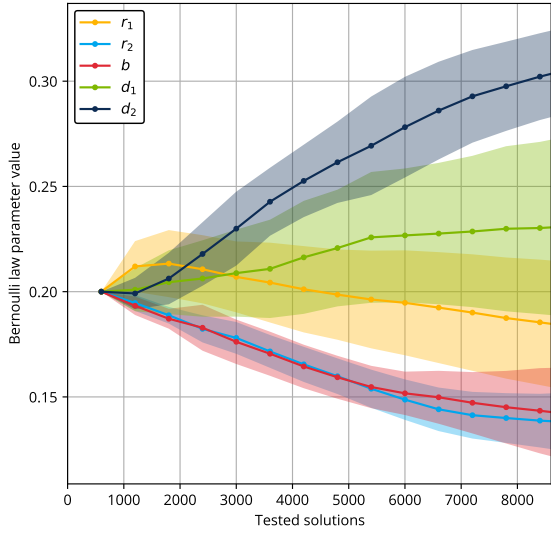
Figure 4: Evolution of mutation rate vector's coordinates during the run, using method AMOW. Interpretations of points and shaded areas are the same as in figure 3.
