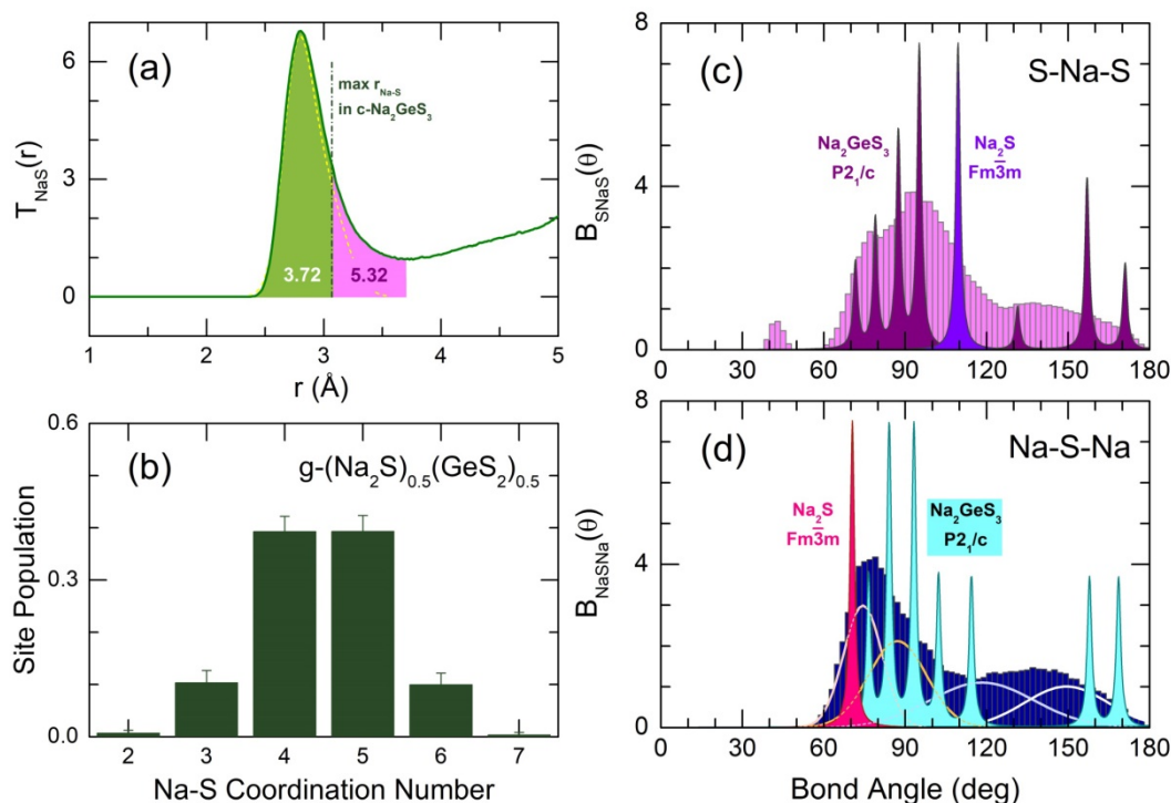
Figure 9. FPMD structural parameters for Na-S subnetwork in glassy (\text{Na}_2\text{S})_{0.5}(\text{GeS}_2)_{0.5} : (a) various approaches to determine sodium coordination environment; the yellow dashed line represents the sum of two Gaussian functions related to Na-S nearest neighbors, the black dash-dotted line shows the maximum Na-S distance in monoclinic \text{Na}_2\text{GeS}_3 ; (b) Na-S coordination distribution, B(\theta) angular distributions for (c) S-Na-S and (d) Na-S-Na bond angles. The B_{\text{SNaS}}(\theta)/B_{\text{NaSNa}}(\theta) functions for crystalline \text{Na}_2\text{GeS}_3 and \text{Na}_2\text{S} are also shown.
