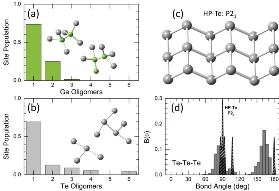
Fig. 7 Gallium and tellurium oligomers in g\text{-Ga}_2\text{Te}_3 : the size distribution of (a) \text{Ga}_n and (b) \text{Te}_n oligomers, (c) structural motif of high-pressure monoclinic HP-Te II, space group P2_1 , 67 (d) the bond angle distribution B_{\text{TeTeTe}}(\theta) in \text{Te}_3 and higher \text{Te}_n oligomers, n > 3 , in comparison with that for HP-Te II. The insets show typical shapes of \text{Ga}_n and \text{Te}_n oligomers.
