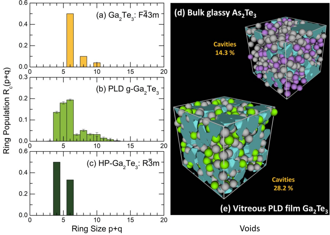
Fig. 8 Rings and cavities in vitreous \text{Ga}_2\text{Te}_3 . Ring statistics R_c(p+q) 39 in (a) ambient pressure cubic, 11 (b) glassy (this work), and (c) high-pressure rhombohedral 52 \text{Ga}_2\text{Te}_3 polymorphs. Cavities in (d) bulk glassy \text{As}_2\text{Te}_3 (preliminary results) and (e) vitreous \text{Ga}_2\text{Te}_3 PLD thin film.
