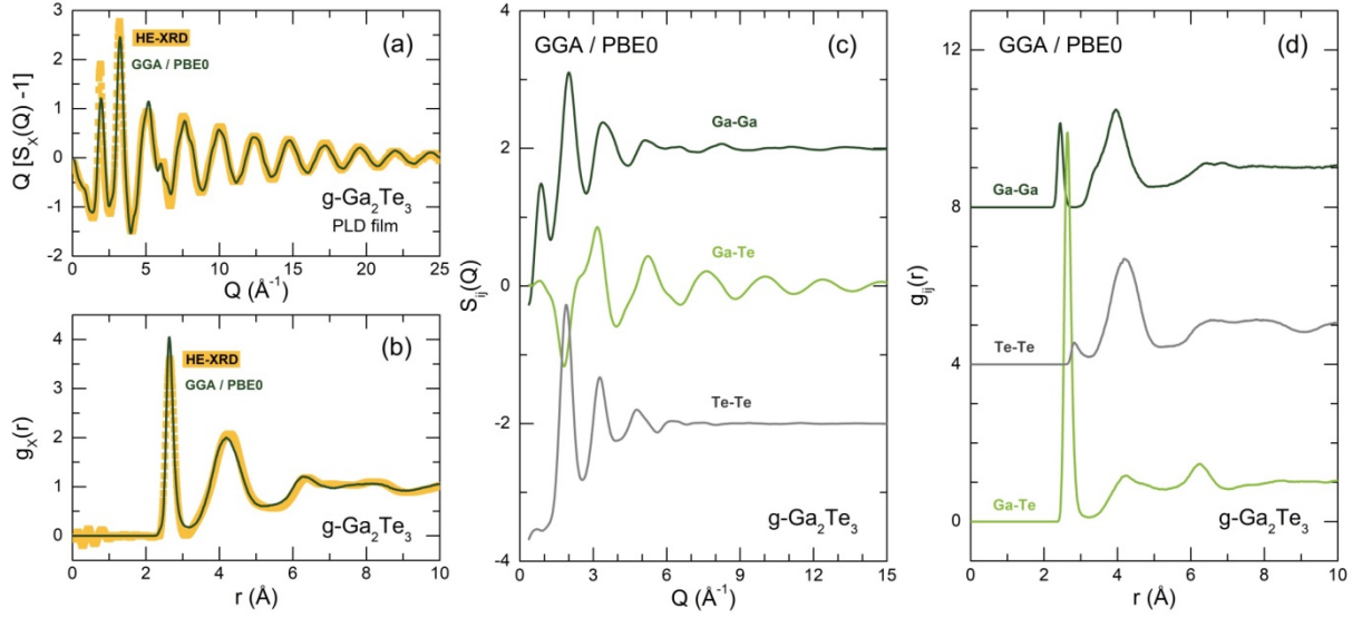
Fig. 4 GGA/PBE0 simulation results for vitreous \text{Ga}_2\text{Te}_3 PLD film. Experimental and simulated (a) X-ray interference function Q[S_X(Q) - 1] and (b) pair-distribution function g_X(r) ; (c) partial Faber-Ziman structure factors S_{ij}(Q) ; and (d) partial pair-distribution functions g_{ij}(r) .
