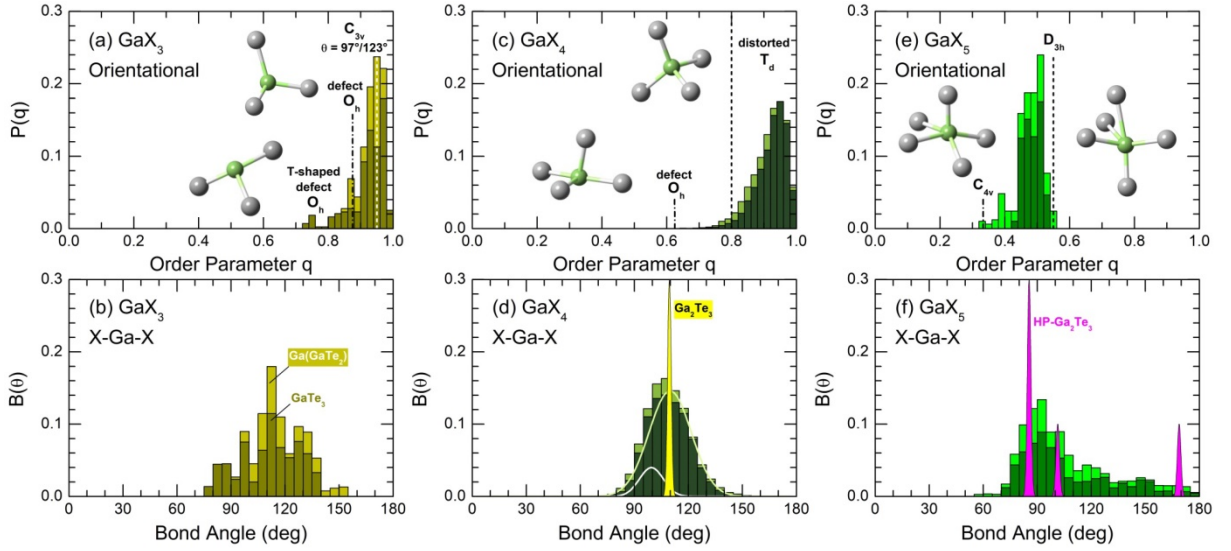
Fig. 6 Orientational order parameter q and X-Ga-X bond angle distribution B_{\text{XGaX}}(\theta) , where X = \text{Te} or \text{Ga} for (a,b) \text{GaX}_3 , (c,d) \text{GaX}_4 , and (e,f) \text{GaX}_5 polyhedra. The insets show typical shapes of Ga-Te entities. The B_{\text{TeGaTe}}(\theta) distributions for cubic (yellow) and rhombohedral (magenta) \text{Ga}_2\text{Te}_3 are also shown. The parameters of pure heteropolar units \text{GaTe}_3 , \text{GaTe}_4 and \text{GaTe}_5 are highlighted in dark colors; their mixed counterparts are pale-colored.
