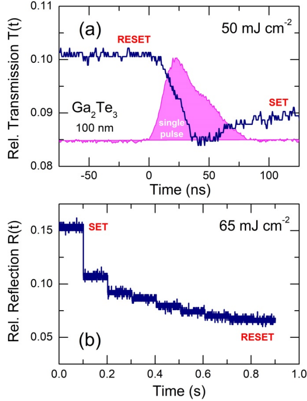
Fig. 10 Optical SET-RESET transitions in Ga 2 Te 3 PLD films (100 nm) induced by a nanosecond laser with \lambda_{\text{pump}} = 532 nm: (a) a single pulse with the energy density 50 \text{ mJ cm}^{-2} (transmission mode); (b) a multi-pulse train with the energy density 65 \text{ mJ cm}^{-2} (reflection mode) and the repetition rate 10 Hz.
