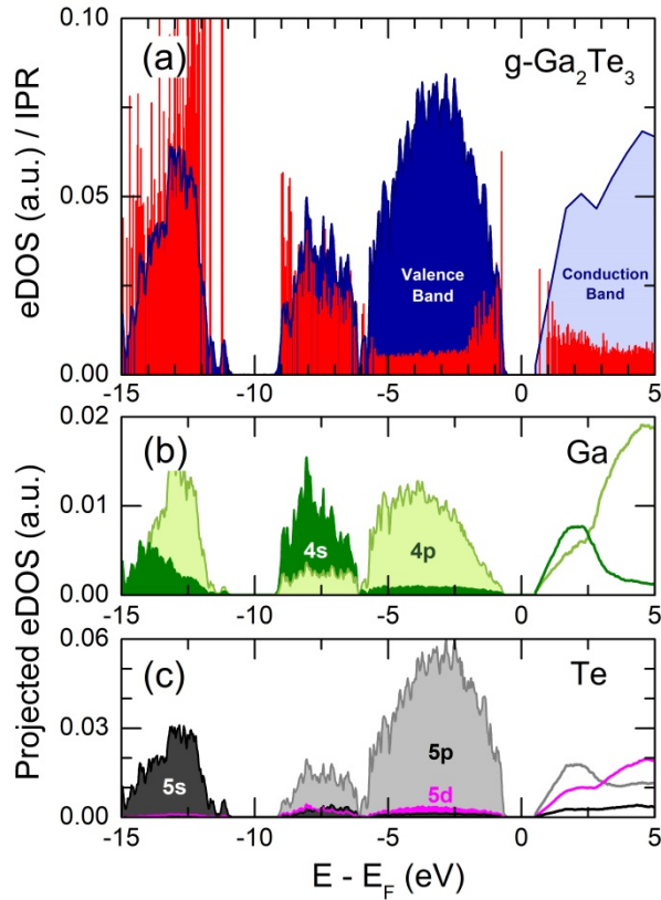
Fig. 9 Electronic properties of glassy Ga 2 Te 3 : (a) the electronic density of states (eDOS) and the inverse participation ratio (IPR, red spikes); the projected eDOS on (b) Ga s and p , and (c) Te s , p and d atomic pseudo-wave functions. See text for further details.
