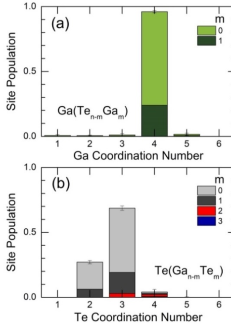
Fig. 5 GGA/PBE0 calculated (a) gallium and (b) tellurium local coordination numbers. Light green and light gray colors highlight pure Ga-Te and Te-Ga fractions in \text{Ga}(\text{Te}_{n-m}\text{Ga}_m) or \text{Te}(\text{Ga}_{n-m}\text{Te}_m) polyhedra ( m = 0 ), respectively. Dark green and dark gray tones correspond to m = 1 . Bright red and blue colors denote populations of Te-rich homopolar \text{Te}(\text{Ga}_{n-m}\text{Te}_m) units, m \geq 2 .
