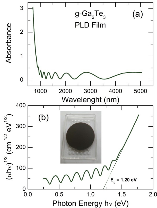
Fig. 1 Optical properties of vitreous Ga 2 Te 3 PLD film: (a) optical absorbance with interference fringes, (b) the Tauc plot: \sqrt{\alpha h\nu} vs photon energy h\nu , where \alpha is the absorption coefficient, used to determine the optical band gap E_g . The inset shows a typical appearance of the Ga 2 Te 3 PLD film.
