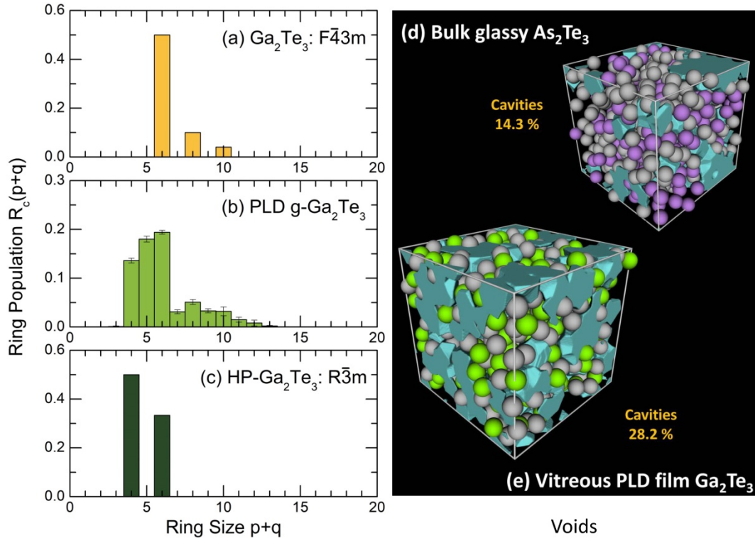
Fig. 8 Rings and cavities in vitreous Ga 2 Te 3 . Ring statistics R_c(p+q) 39 in (a) ambient pressure cubic, 11 (b) glassy (this work), and (c) high-pressure rhombohedral 52 Ga 2 Te 3 polymorphs. Cavities in (d) bulk glassy As 2 Te 3 (preliminary results) and (e) vitreous Ga 2 Te 3 PLD thin film.
