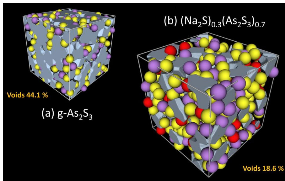
Figure 12. Cavities in (a) g\text{-As}_2\text{S}_3 49 and (b) g\text{-(Na}_2\text{S)}_{0.3}\text{(As}_2\text{S}_3)_{0.7} , derived using the pyMolDyn program. 39 The fraction of voids normalized to the simulation box volume has decreased by a factor of 2.4, from 44.1 % to 18.6 %, for the sodium thioarsenate glass.
