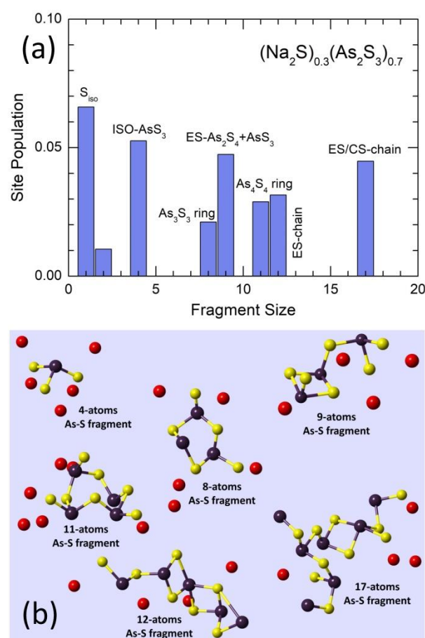
Figure 10. Small As-S fragments forming a disconnected As-S subnetwork in g\text{-}(\text{Na}_2\text{S})_{0.3}(\text{As}_2\text{S}_3)_{0.7} : (a) statistics of small As-S units, and (b) typical examples present in the FPMD simulation box.
