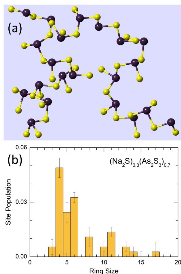
Figure 11. (a) 60-atoms long As-S chain consisting of corner-sharing pyramidal units \text{CS-AsS}_{3/n} , where n = 1, \text{S}(t) , or 2, \text{S}(b) , and (b) the derived ring statistics in glassy (\text{Na}_2\text{S})_{0.3}(\text{As}_2\text{S}_3)_{0.7} .
