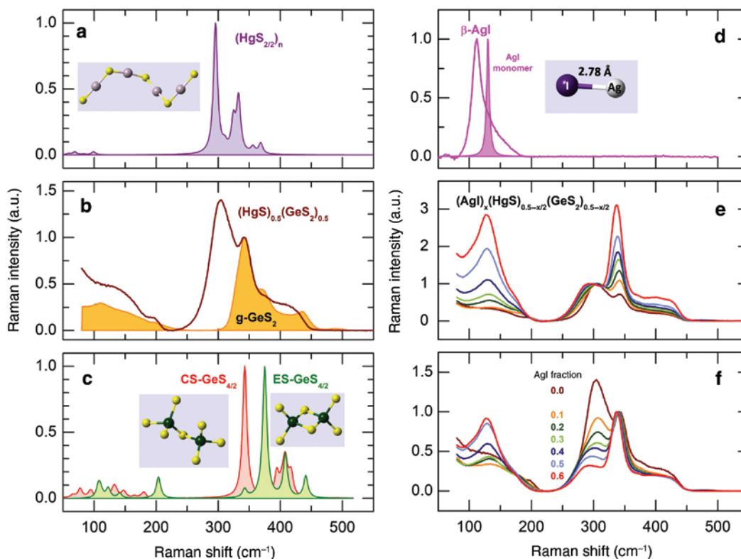
Fig. 4: Experimental and DFT Raman spectra related to AgI-HgS-GeS 2 glasses: (a) DFT chain-like cluster Hg 2 S 5 [17], (b) equimolar glassy host (\text{HgS})_{0.5}(\text{GeS}_2)_{0.5} and glassy GeS 2 , (c) corner- and edge-sharing CS-GeS 4/2 and ES-GeS 4/2 clusters [38], (d) hexagonal \beta -AgI and DFT monomer AgI, selected (\text{AgI})_x(\text{HgS})_{0.5-x/2}(\text{GeS}_2)_{0.5-x/2} glasses normalised to (e) the Hg-S symmetric stretching mode at 300 cm -1 , or to (f) the Ge-S breathing mode in CS-GeS 4/2 tetrahedra at 340 cm -1 .
