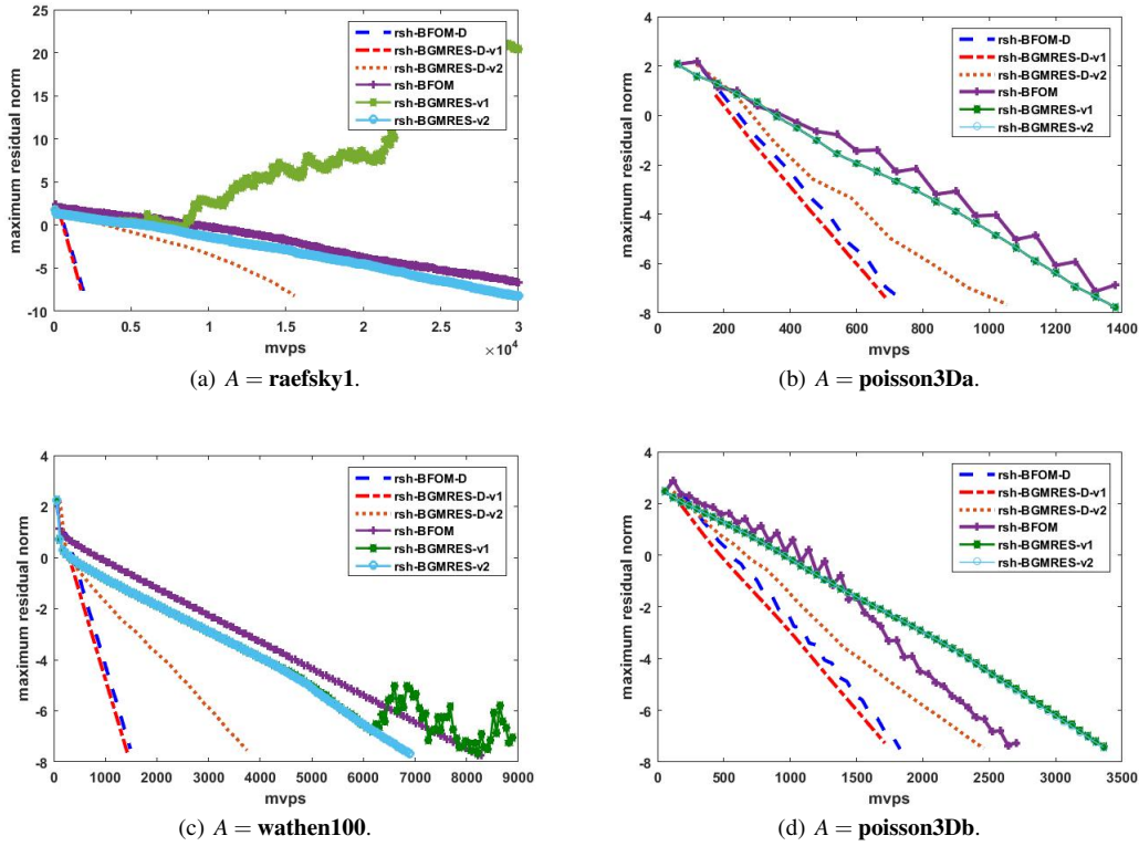
Fig. 2 The \log_{10} plot of the maximum residual norms with respect to the number of matrix-vector products for Example 4 with s = 3 , m = 20 , k = 3 and l = 3 .
