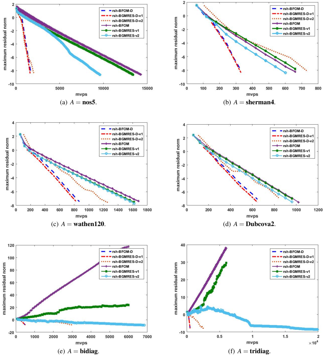
Fig. 1 The \log_{10} plot of the maximum residual norms with respect to the number of matrix-vector products for Example 2 with s = 3 , m = 20 , k = 3 and l = 15 .
