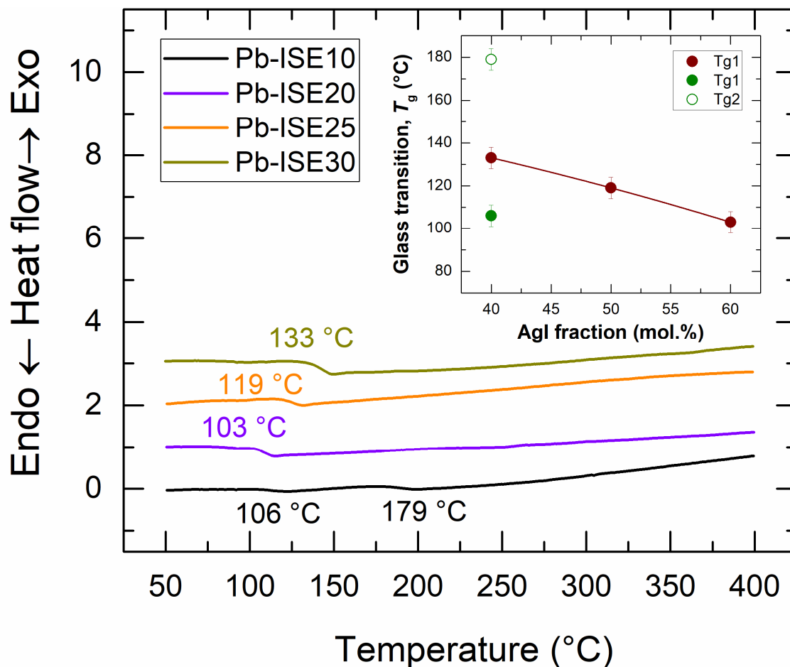
Figure 3. DSC traces of the four glass compositions, obtained by melt quenching, used as active membranes in the lead chemical sensors. The inset shows the evolution of the glass transition temperature as a function of silver iodide molar fraction. The line in the inset is drawn as guide to the eyes.
