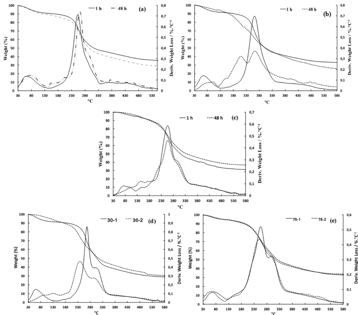
Figure 5. TGA/DTG thermograms of flaxseed gums extracted during 1 h and 48 h at 25 °C (a), at 40 °C (b), at 70 °C (c) and by UAE during 30 min (d) and 75 min (e) for stages 1 and 2.
