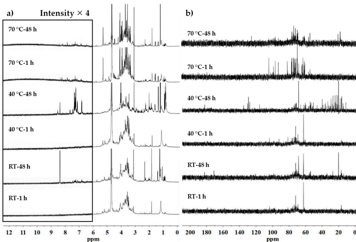
Figure 1. 1 H (a) and 13 C (b) NMR spectra of flaxseed mucilage extracted by magnetic stirring method depending on time and temperature.
