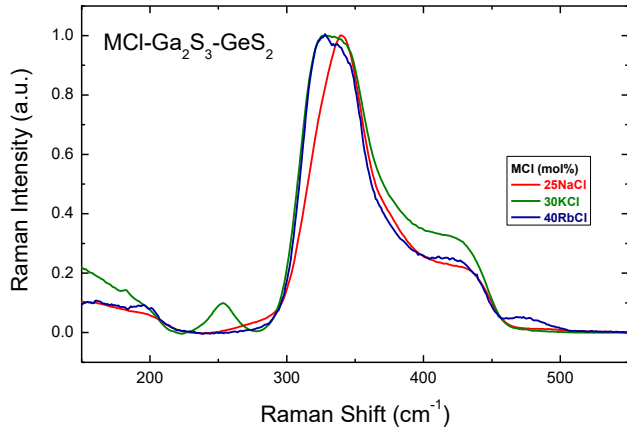
Fig. 9: Experimental Raman spectra of (MCl)_x(Ga_2S_3)_{0.2-0.2x}(GeS_2)_{0.8-0.8x} glasses: x = 25 for M = Na ; x = 30 for M = K ; x = 40 for M = Rb .
