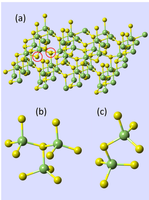
Fig. 8: Lattice and structural motifs in monoclinic \text{Ga}_2\text{S}_3 [29]: (a) selected two-fold \text{S}_{2\text{F}} and three-fold \text{S}_{3\text{F}} coordinated sulfur species in the lattice are indicated by red circles, (b) a Ga-S tricluster, (c) a corner-sharing \text{CS-Ga}_2\text{S}_7 dimer.
