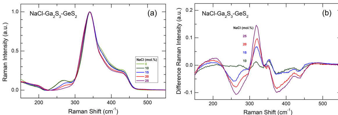
Fig. 1: (a) Experimental Raman spectra of (\text{NaCl})_x(\text{Ga}_2\text{S}_3)_{0.2-0.2x}(\text{GeS}_2)_{0.8-0.8x} glasses, 0.0 \leq x \leq 0.25 ; (b) the difference Raman spectra of NaCl-containing glasses obtained by subtraction of the spectrum for vitreous matrix (\text{Ga}_2\text{S}_3)_{0.2}(\text{GeS}_2)_{0.8} .
