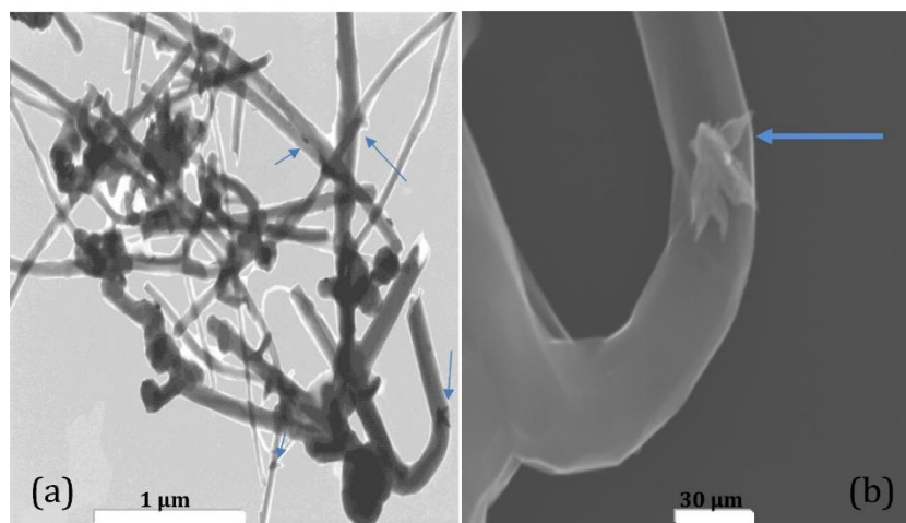
Figure 5 TEM micrographs of the Pd-Cu/MWCNTs: a) 1 μm resolution and b) 100 μm resolution.
