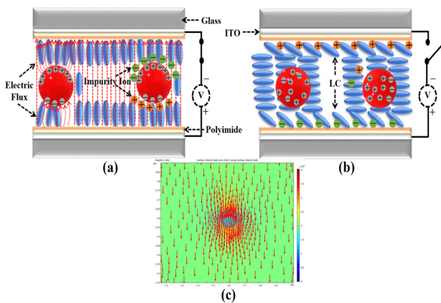
Fig. 7 (a) Schematic representation illustrating the functioning of NLCs in an on state NLC cell doped with SnSe NSs. (b) Schematic depiction illustrating the functioning of NLCs in an off state NLC cell doped with SnSe NSs and (c) the calculated distribution of an electric field in a NS surrounded by LC molecules. The electric field direction is indicated by the red arrow, while the color represents the field strength.
