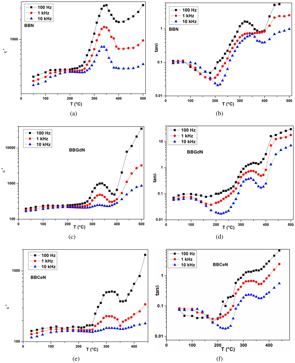
Fig. 3. Temperature dependence of dielectric constant \epsilon' and loss tangent \tan\delta of Ln-doped BaBi_2Nb_2O_9 ceramics.
