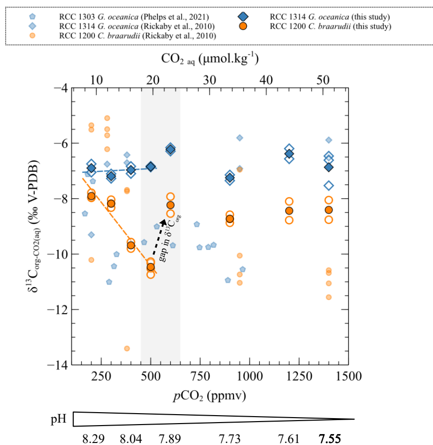
330 Figure 7: Carbon isotopic ratios of organic matter compared to \delta^{13}\text{C}_{\text{CO}_2\text{aq}} of the strains studied with changes in CO 2 level and pH. The empty points are all the replicate data and the filled points are the means. The grey band represents the carbonate chemistry condition where a shift in the carbon and oxygen isotope ratio occurs. The sources of previously reported data (smaller symbols) are inset.
