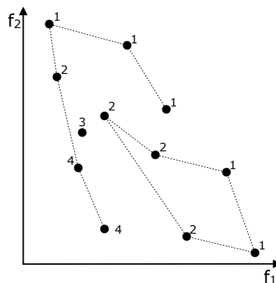
PLOS-net [PPSN'18]
